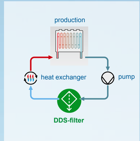
ethylen-glycol refrigeration circuit
