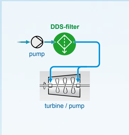
filtration of sealing water
