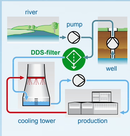
filtration of additional water
